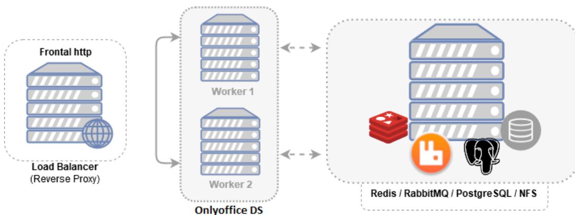
Figure 2: Infrastructure Onlyoffice
