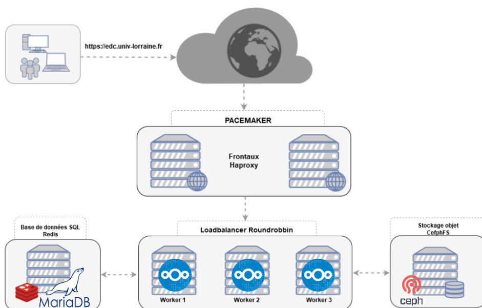
Figure 1: Infrastructure Nextcloud
